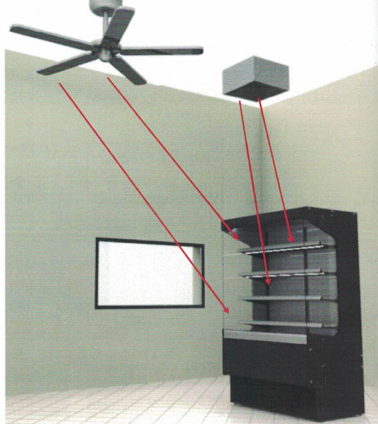
HVAC ceiling vents and ceiling fans will effect the airflow of open showcases and could create condensation on the glass of closed showcases
