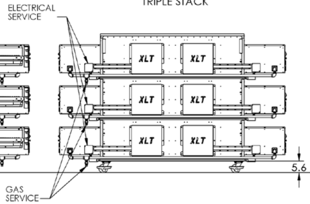
BACK VIEW TRIPLE STACK
